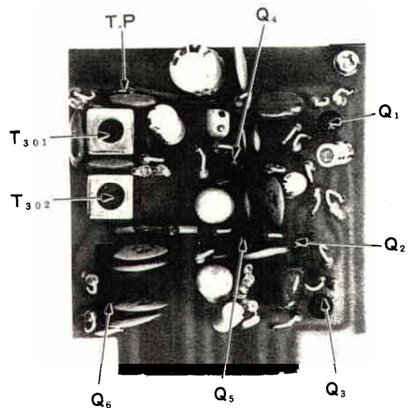
Fig. 22 FM UNIT
